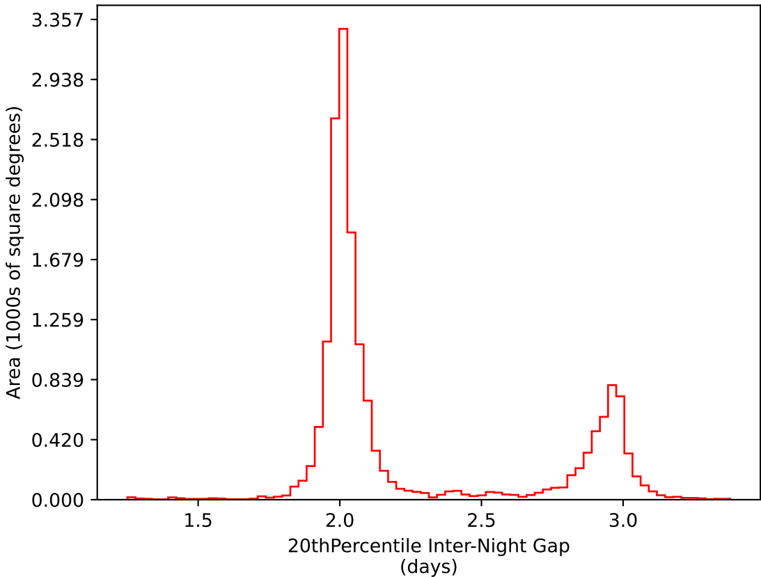
roman_v3.3_10yrs WFD i band: 20thPercentile Inter-Night Gap
