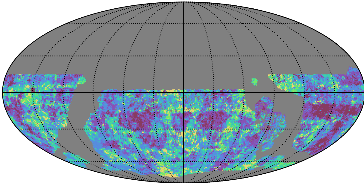
roman_v3.3_10yrs WFD g band: 20thPercentile Inter-Night Gap
