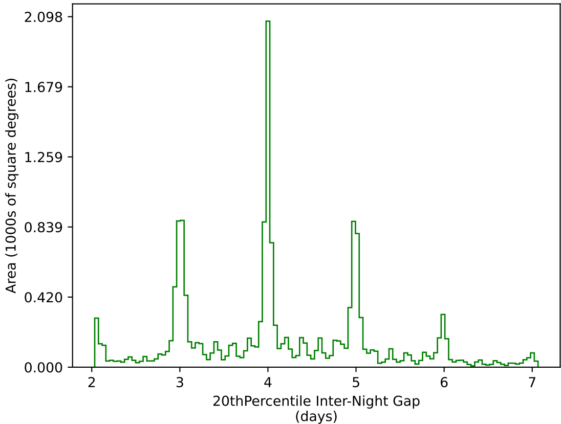
roman_v3.3_10yrs WFD g band: 20thPercentile Inter-Night Gap
