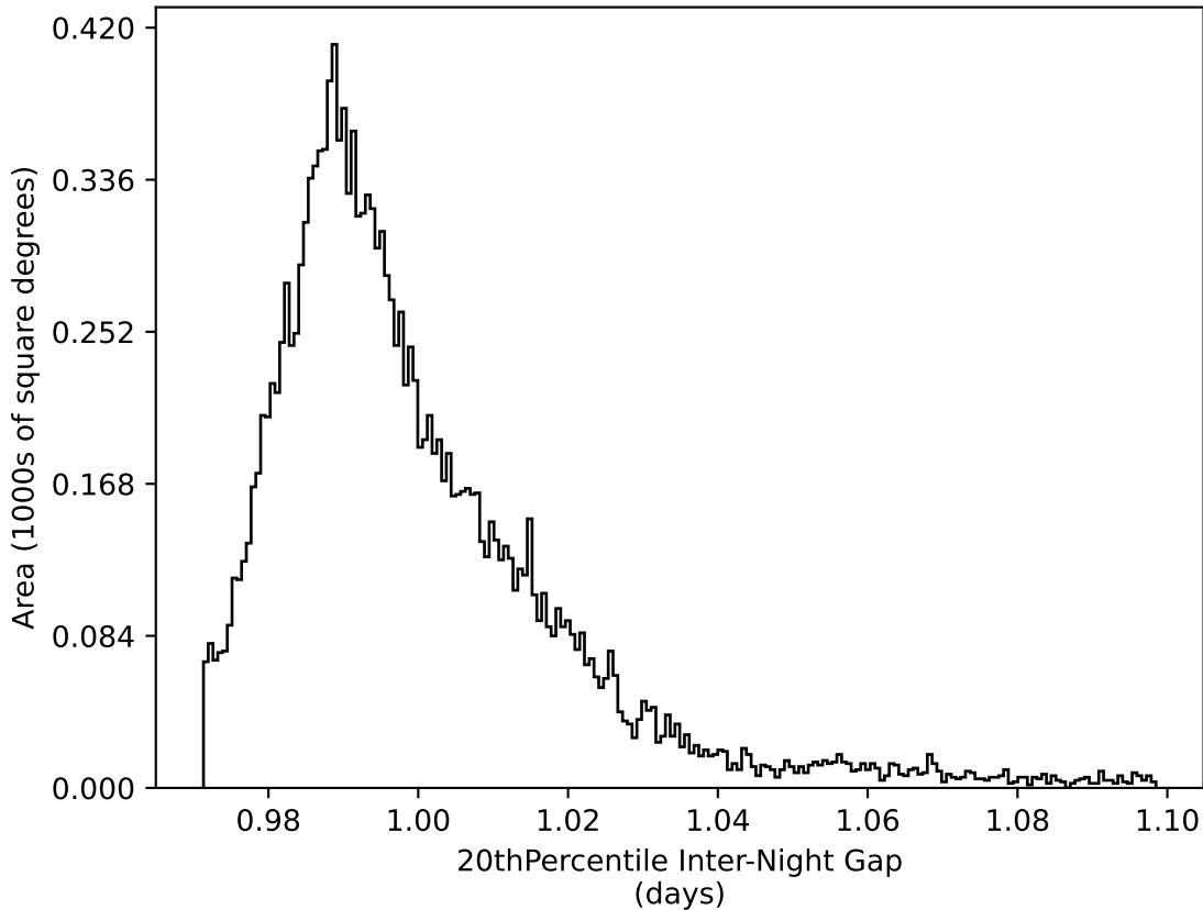
roman_v3.3_10yrs WFD all bands: 20thPercentile Inter-Night Gap
