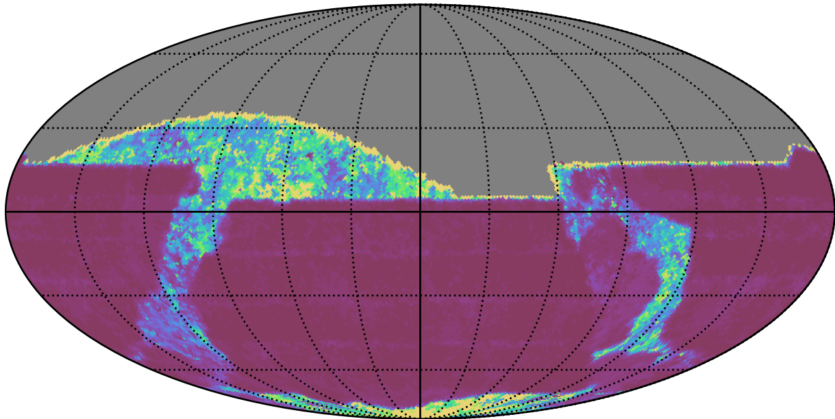
roman_v3.3_10yrs All sky z band: 20thPercentile Inter-Night Gap
