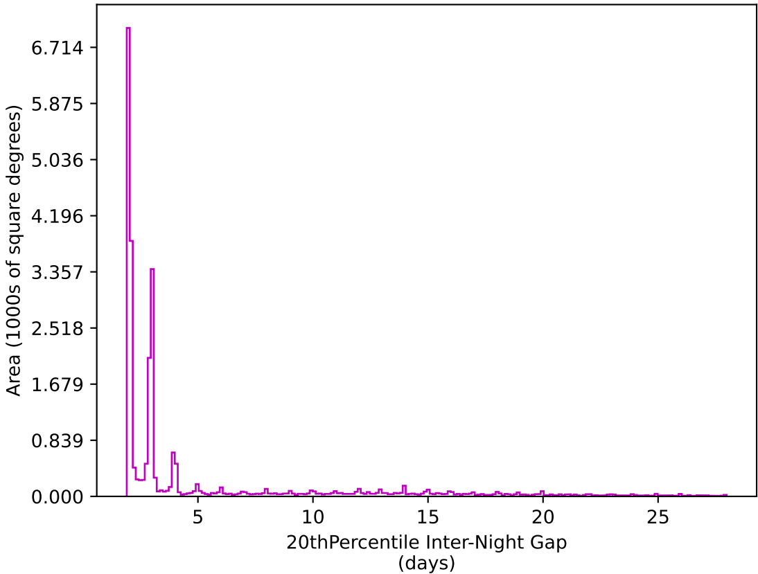
roman_v3.3_10yrs All sky z band: 20thPercentile Inter-Night Gap
