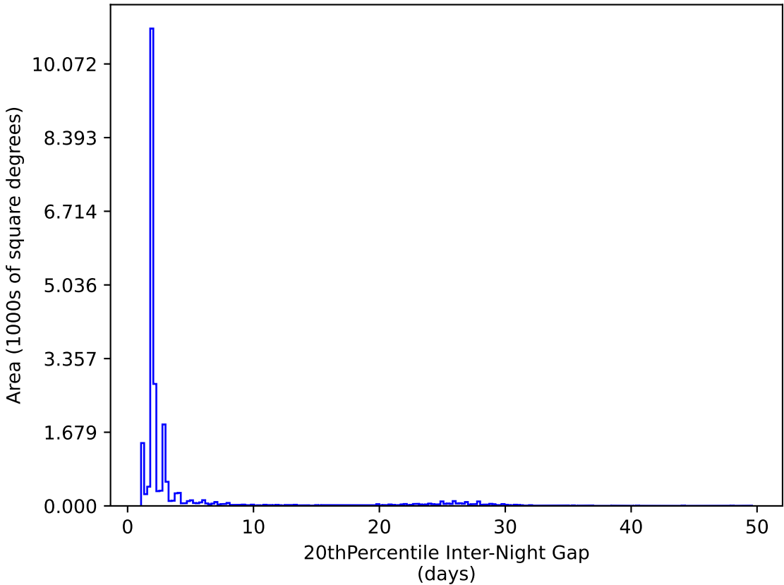
roman_v3.3_10yrs All sky y band: 20thPercentile Inter-Night Gap
