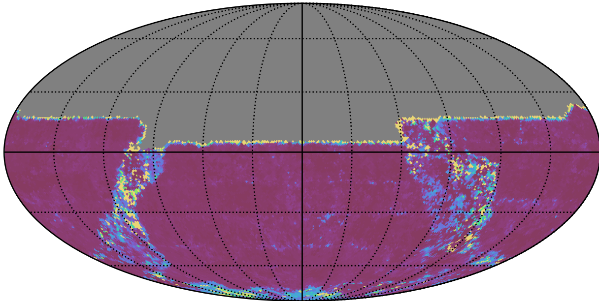
roman_v3.3_10yrs All sky u band: 20thPercentile Inter-Night Gap
