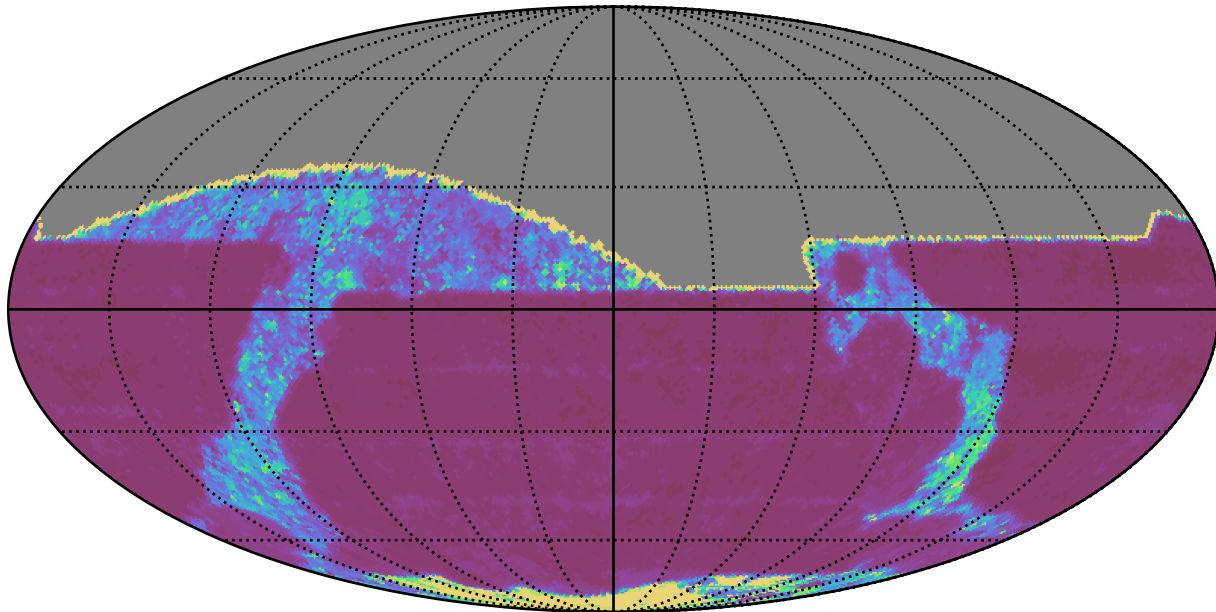
roman_v3.3_10yrs All sky r band: 20thPercentile Inter-Night Gap
