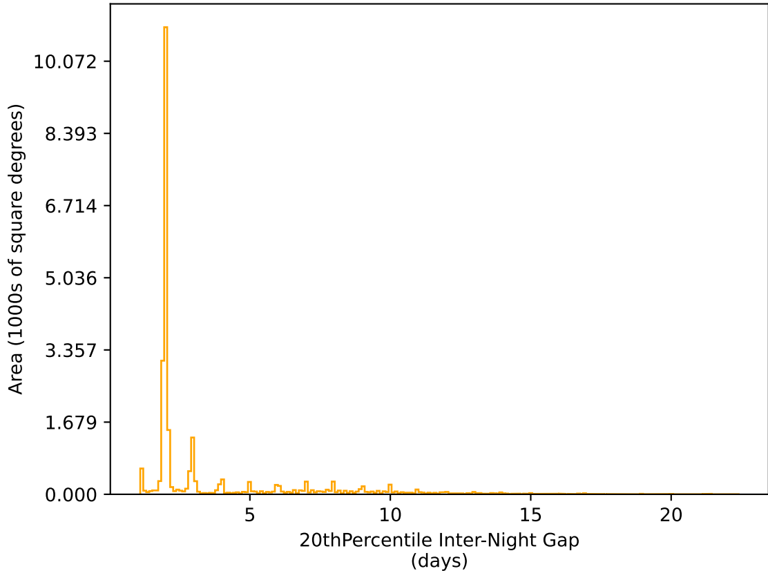
roman_v3.3_10yrs All sky r band: 20thPercentile Inter-Night Gap
