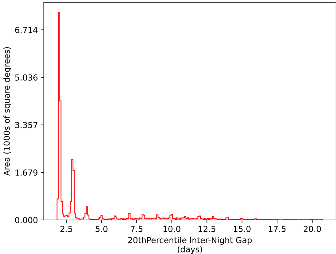
roman_v3.3_10yrs All sky i band: 20thPercentile Inter-Night Gap
