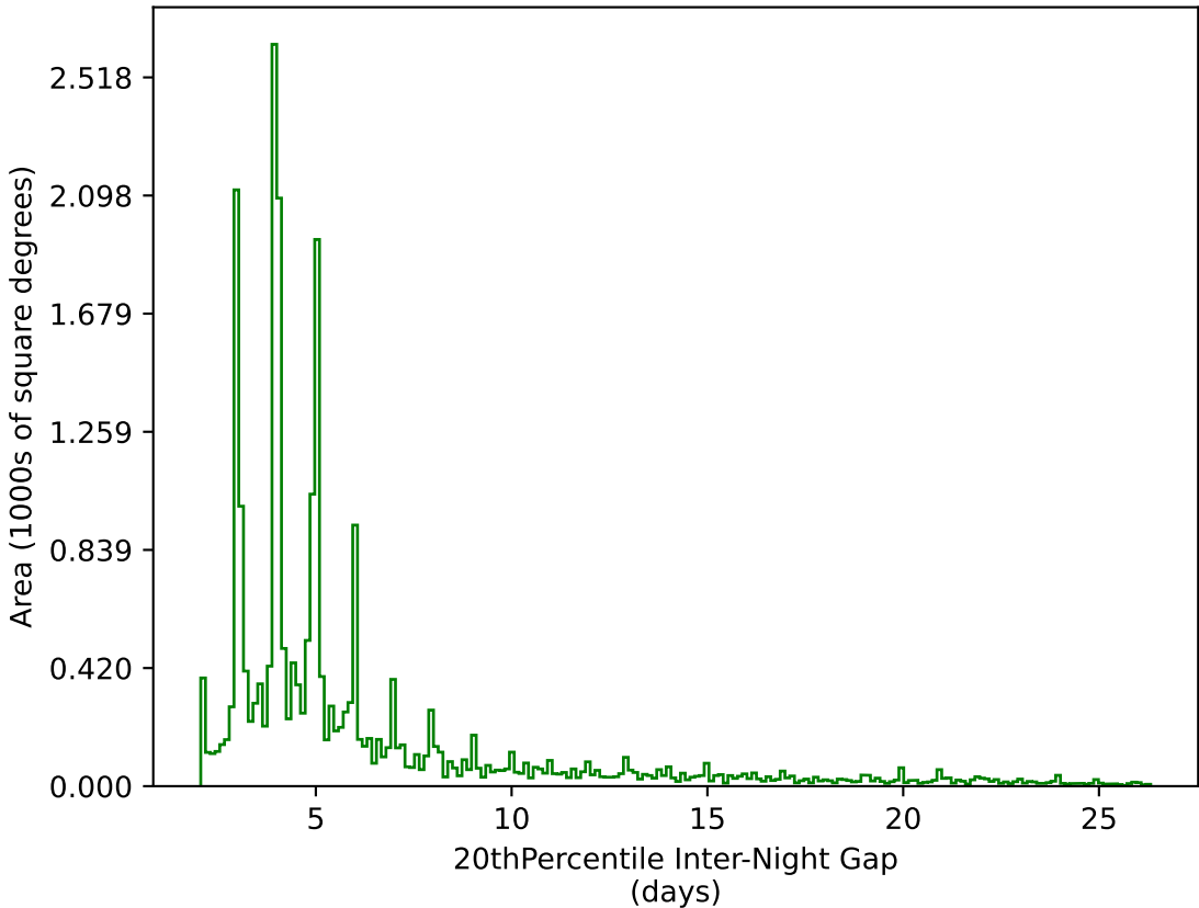
roman_v3.3_10yrs All sky g band: 20thPercentile Inter-Night Gap
