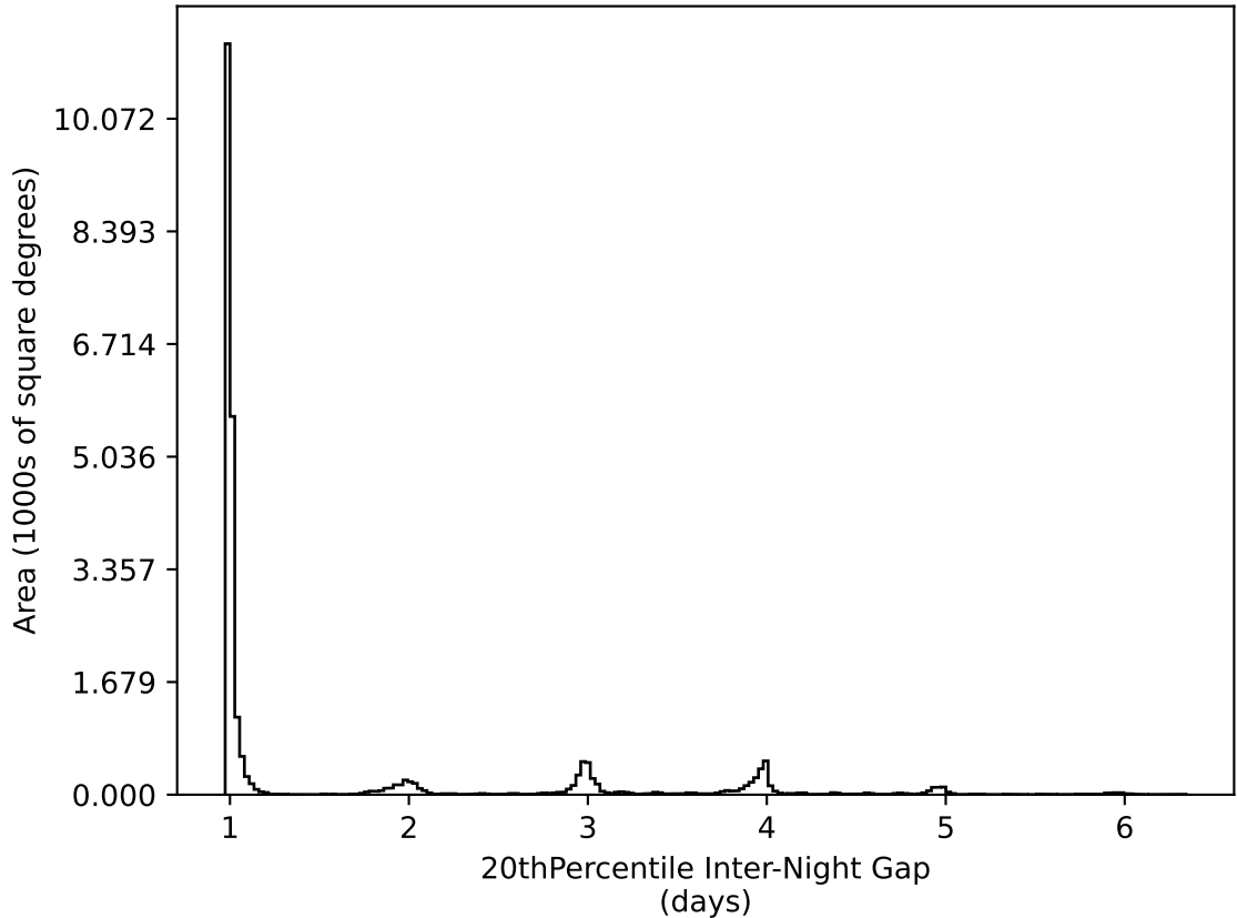
roman_v3.3_10yrs All sky all bands: 20thPercentile Inter-Night Gap
