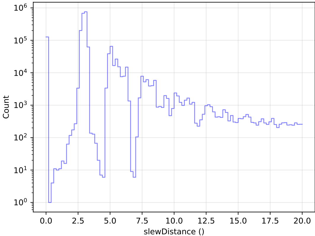
roman_v3.3_10yrs All visits: Zoom Slew Distance Histogram
