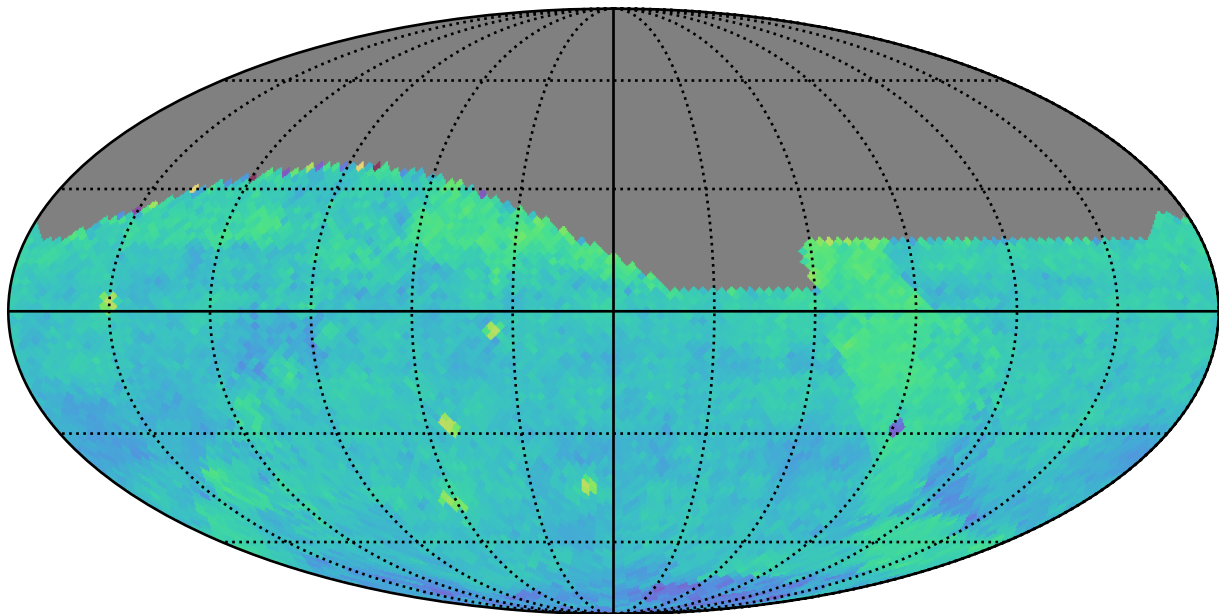
roman_v3.3_10yrs (g or r or i): PairFraction
