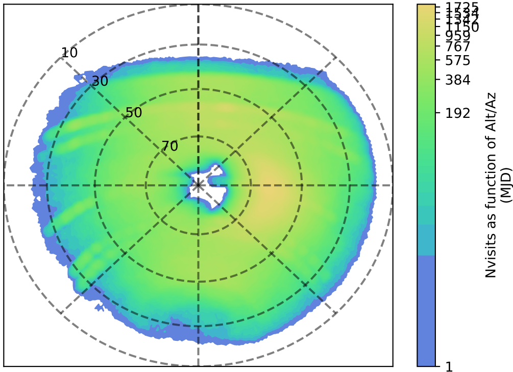
roman_v3.3_10yrs y: Nvisits as function of Alt/Az
