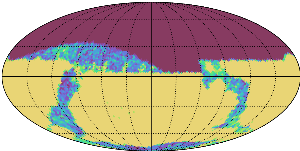
roman_v3.3_10yrs z and night < 365: N year 1
