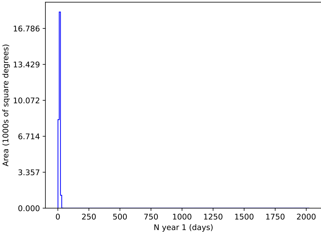
roman_v3.3_10yrs z and night < 365: N year 1
