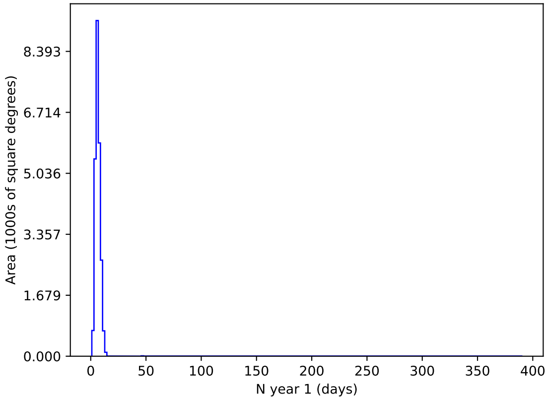
roman_v3.3_10yrs u and night < 365: N year 1
