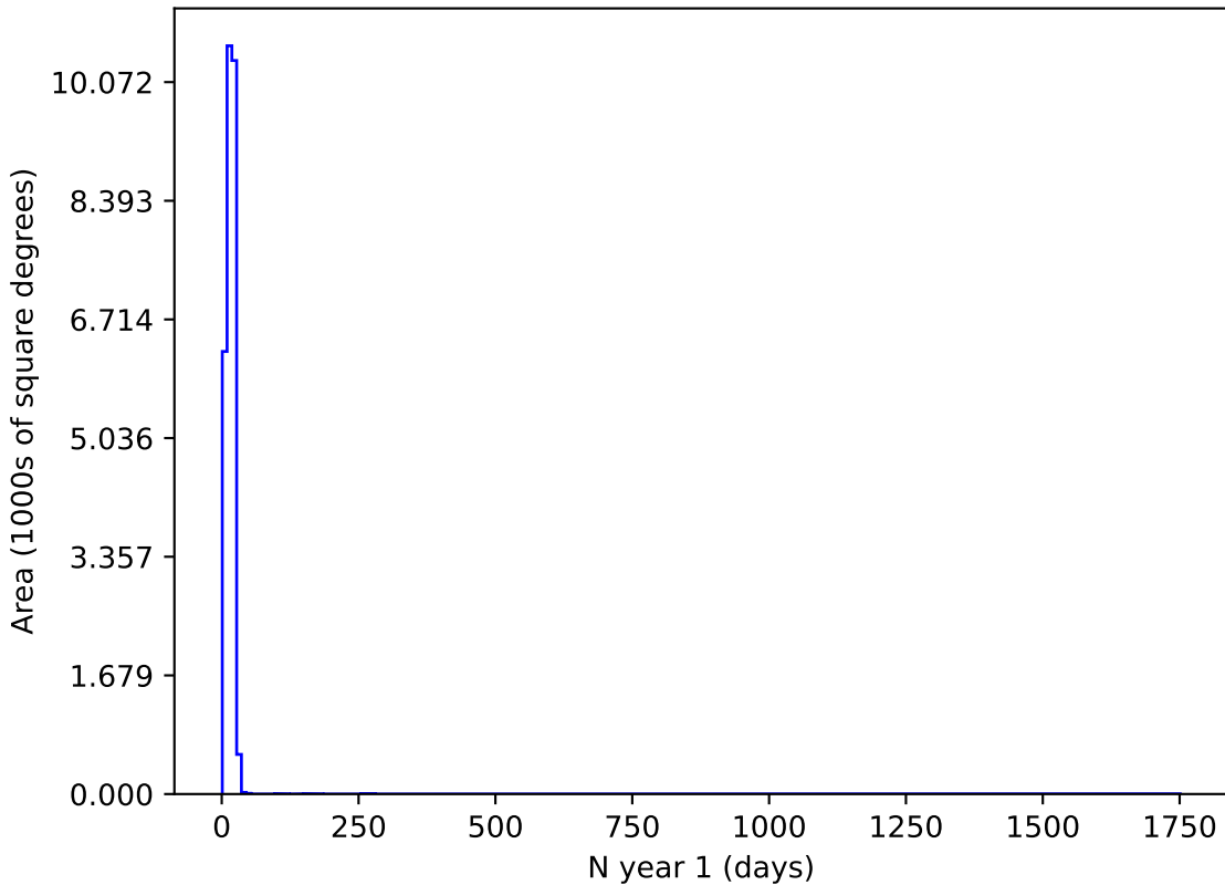
roman_v3.3_10yrs r and night < 365: N year 1
