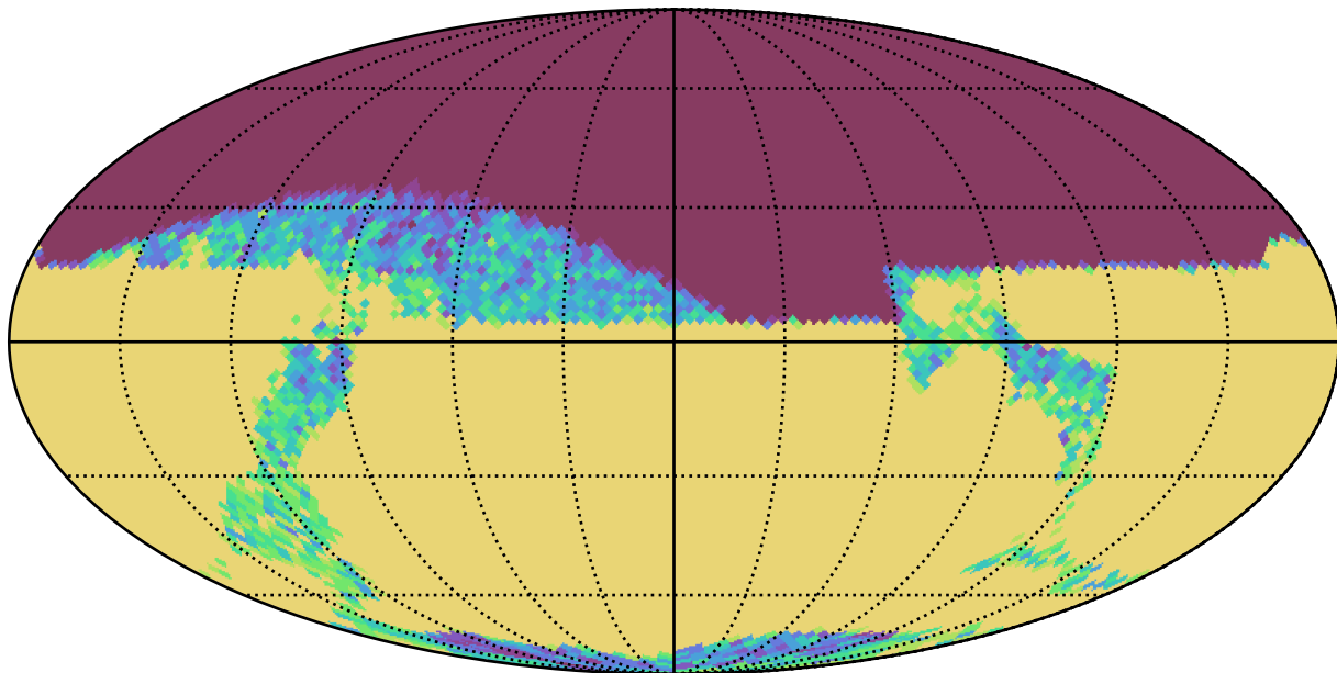
roman_v3.3_10yrs i and night < 365: N year 1
