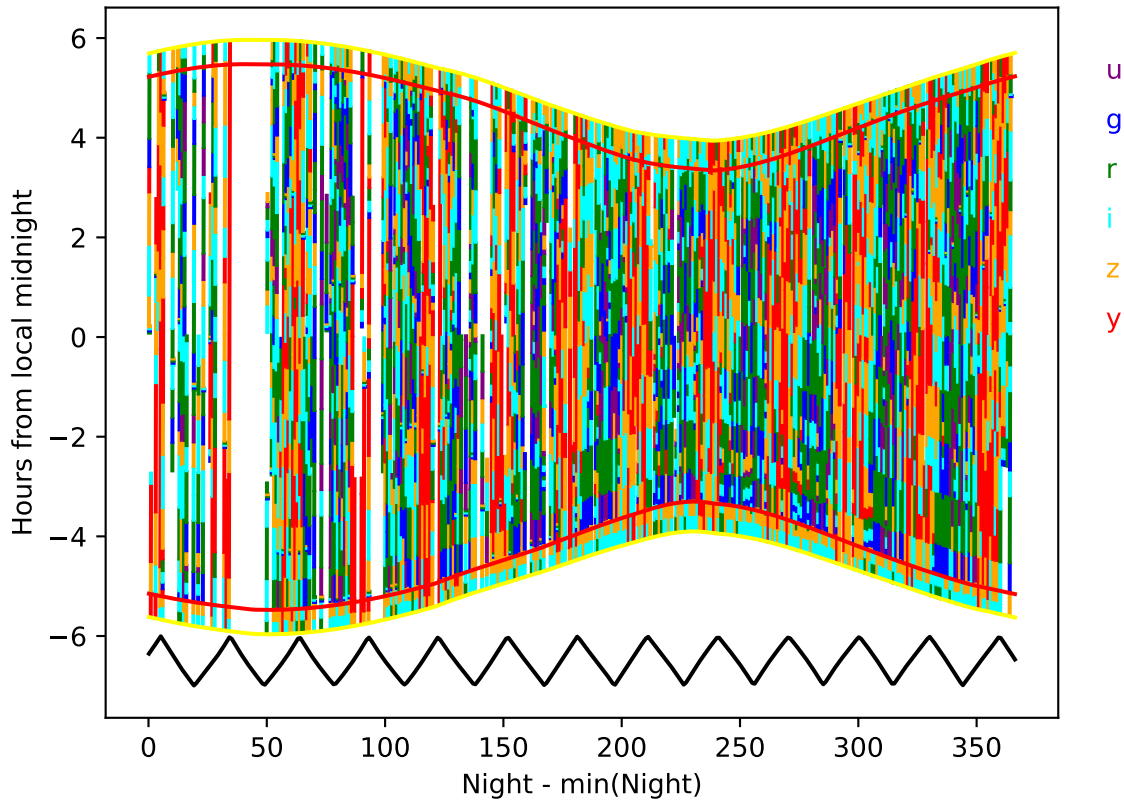
roman_v3.3_10yrs year 6-7: Hourglass
