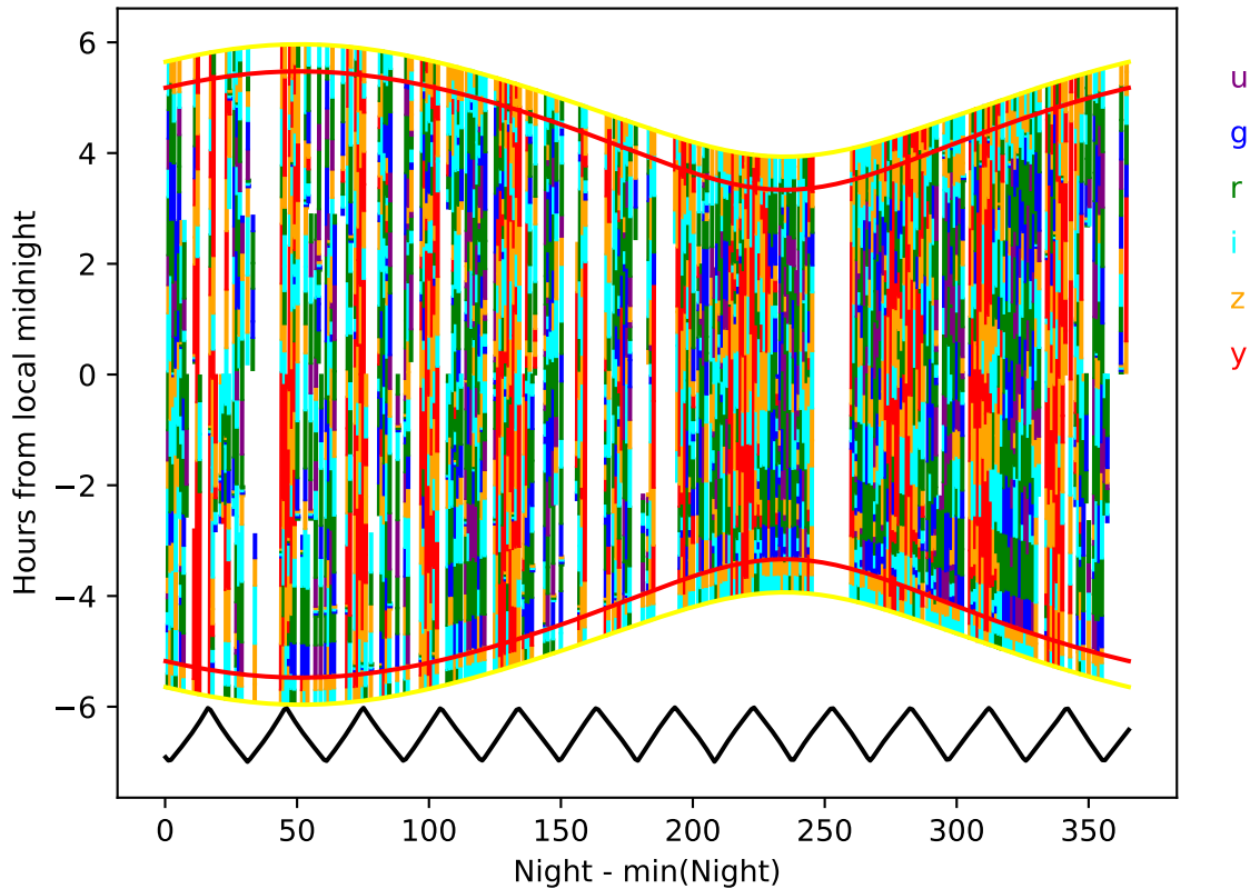
roman_v3.3_10yrs year 5-6: Hourglass
