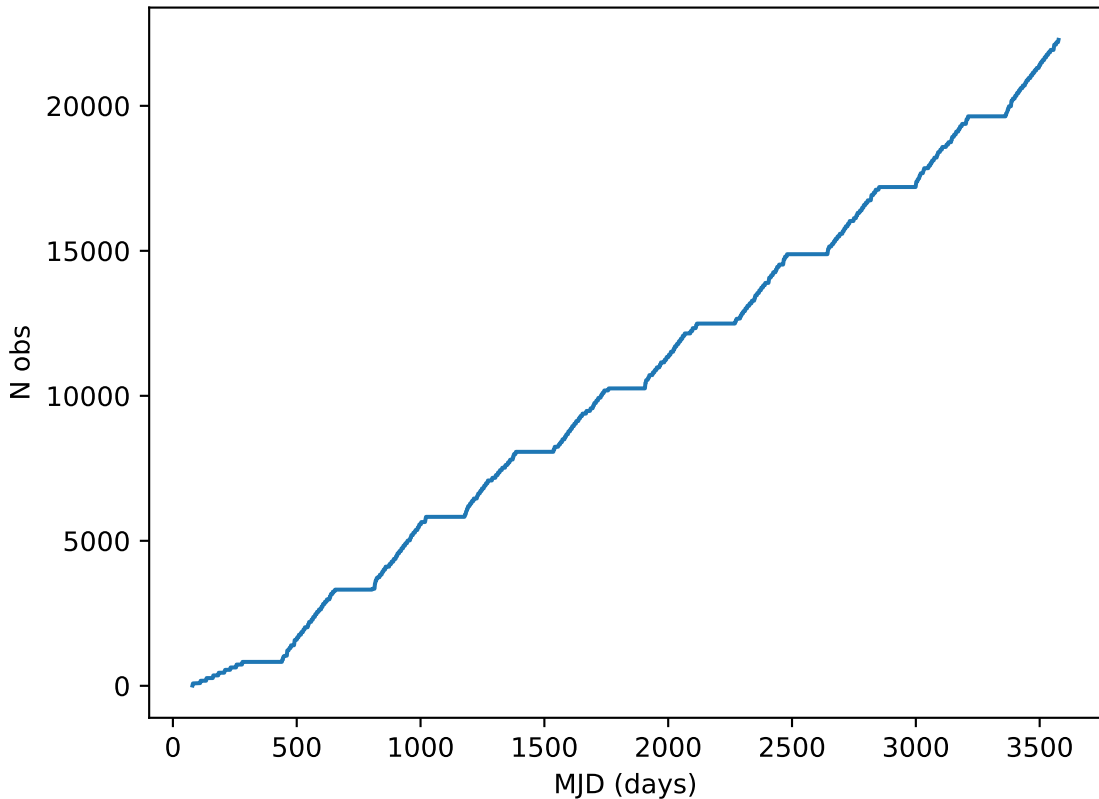
roman_v3.3_10yrs note like DD:XMM_LSS%: Cumulative
