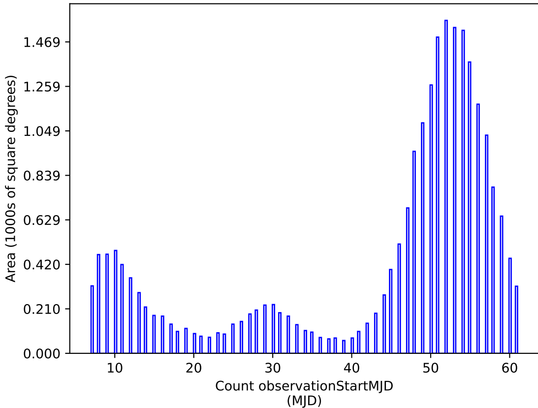
roman_v3.3_10yrs u: Count observationStartMJD
