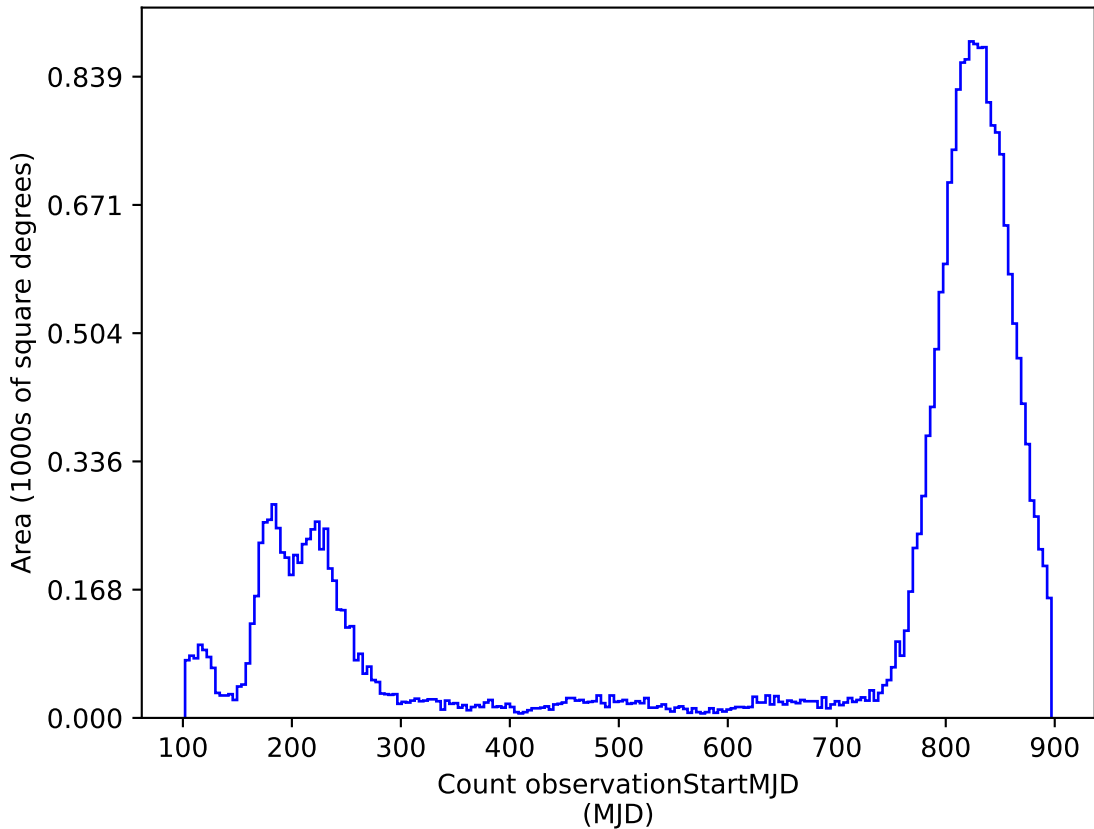
roman_v3.3_10yrs : Count observationStartMJD
