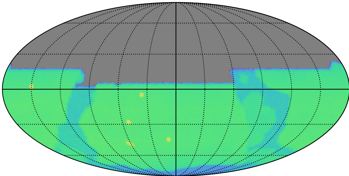
roman_v3.3_10yrs y: CoaddM5
