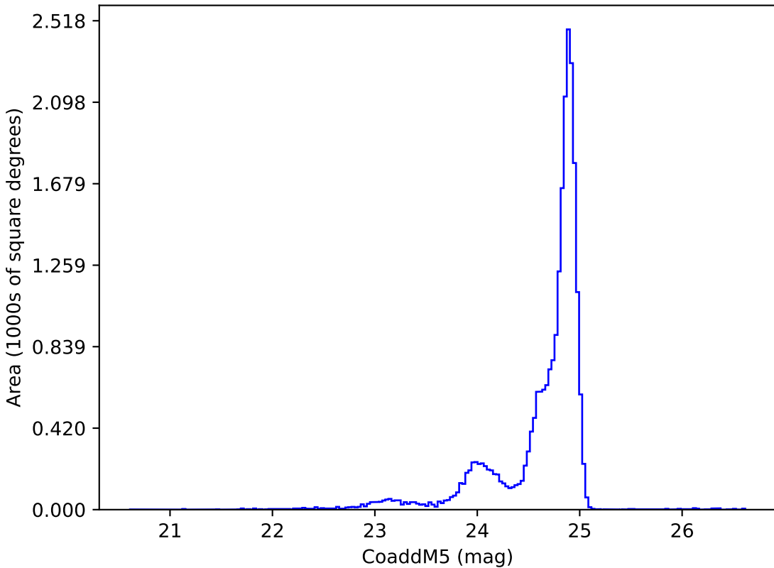
roman_v3.3_10yrs y: CoaddM5
