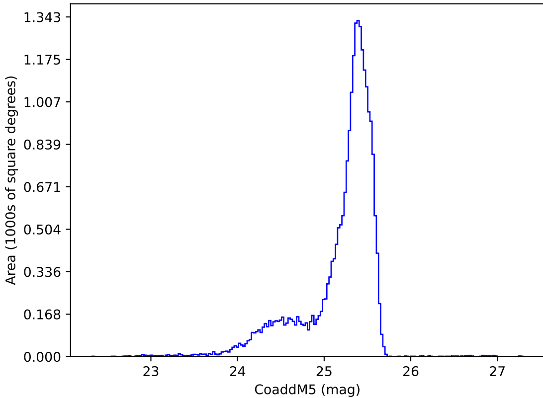
roman_v3.3_10yrs u: CoaddM5
