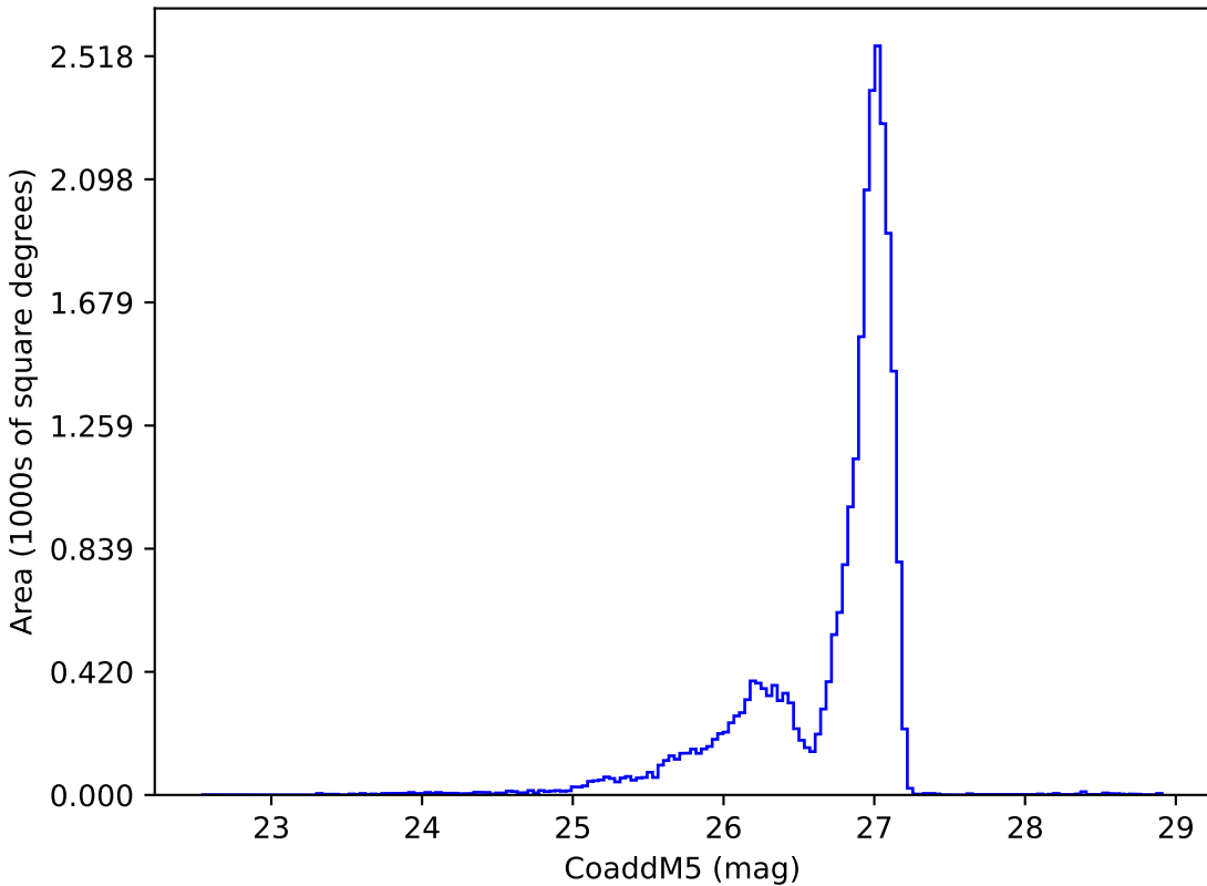
roman_v3.3_10yrs r: CoaddM5
