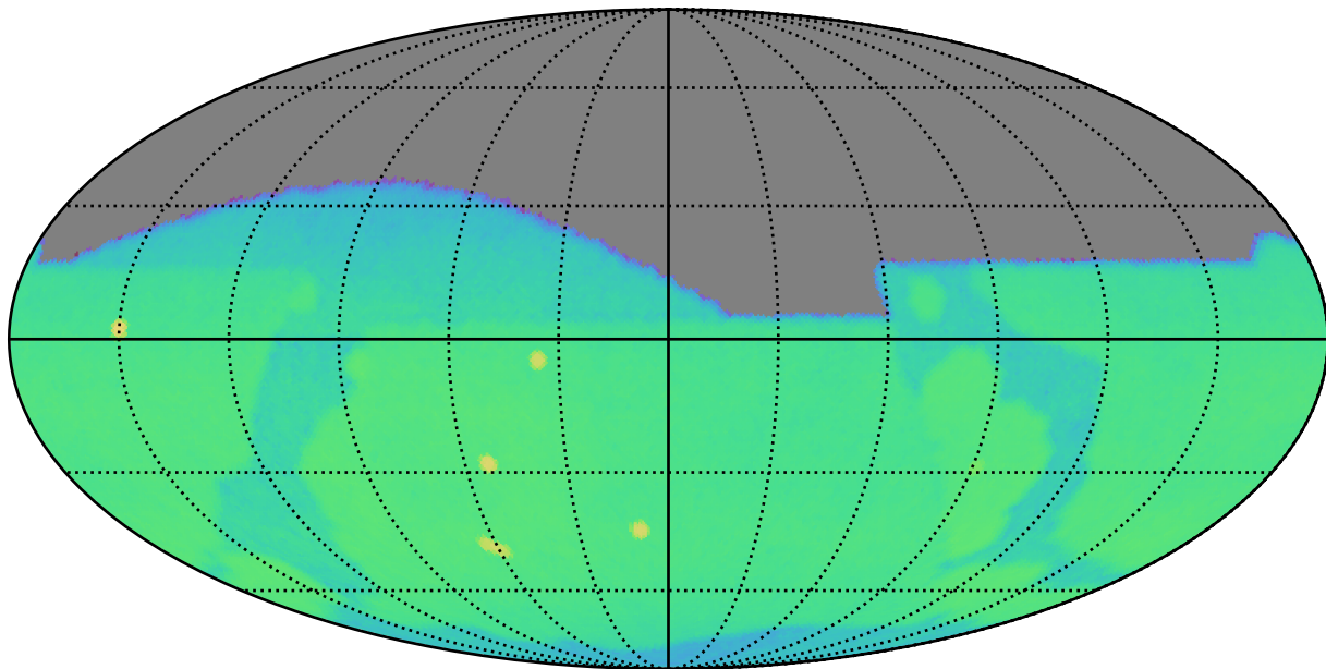
roman_v3.3_10yrs g: CoaddM5
