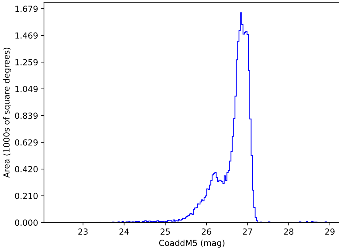
roman_v3.3_10yrs g: CoaddM5
