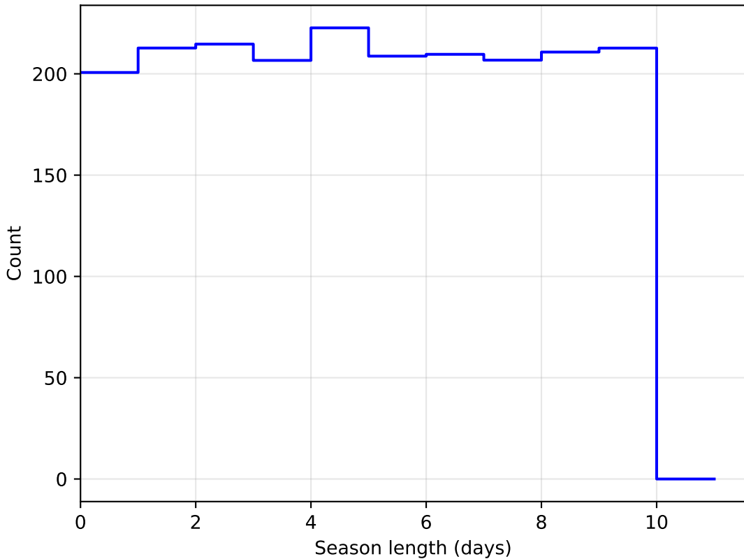
roman_v3.3_10yrs DD:XMM_LSS all bands: SeasonLength
