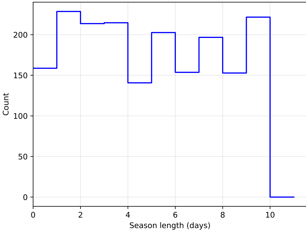
roman_v3.3_10yrs DD:WFD all bands: SeasonLength
