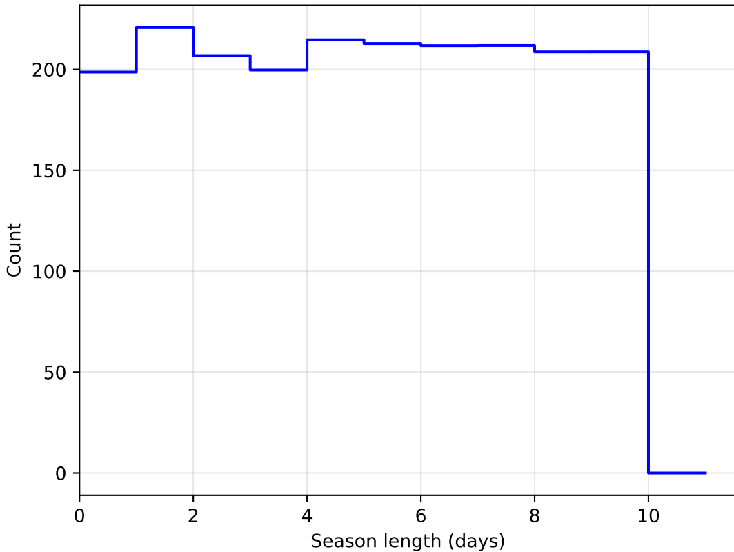
roman_v3.3_10yrs DD:ELAISS1 all bands: SeasonLength
