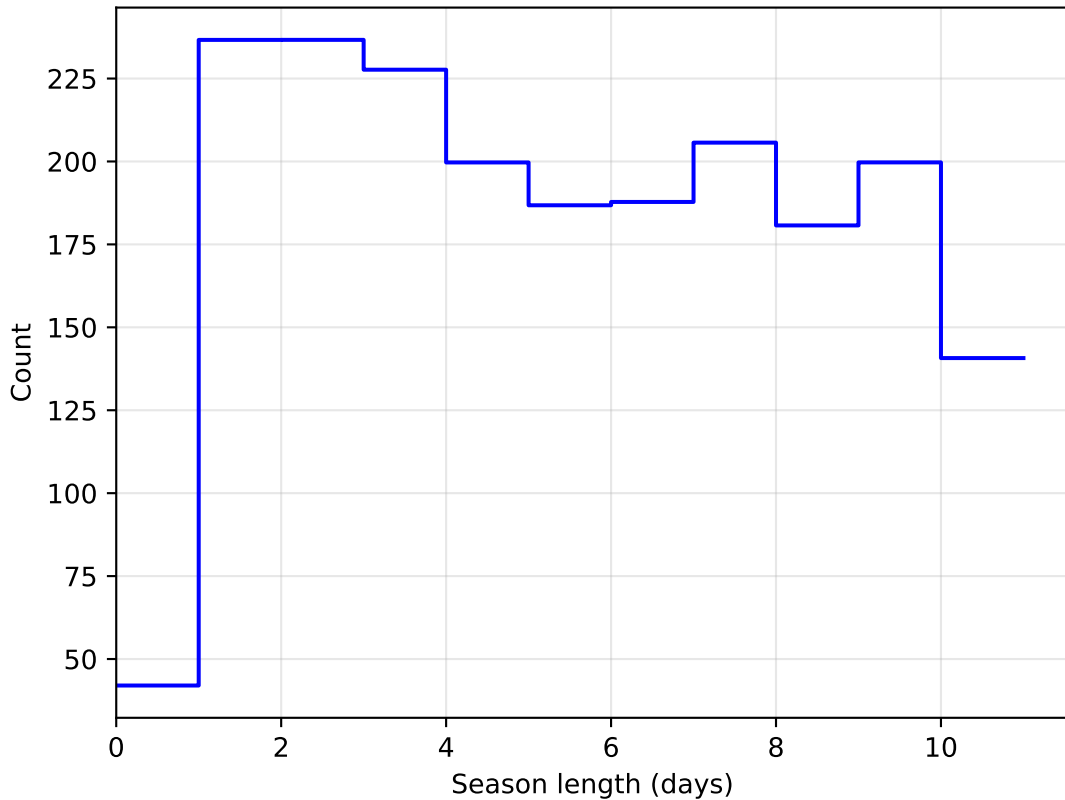
roman_v3.3_10yrs DD: COSMOS all bands: SeasonLength
