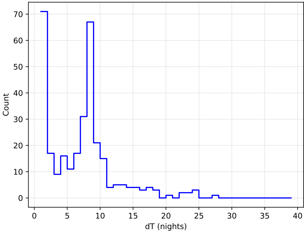
roman_v3.3_10yrs all bands: DD:XMM_LSS Delta Nights Histogram
