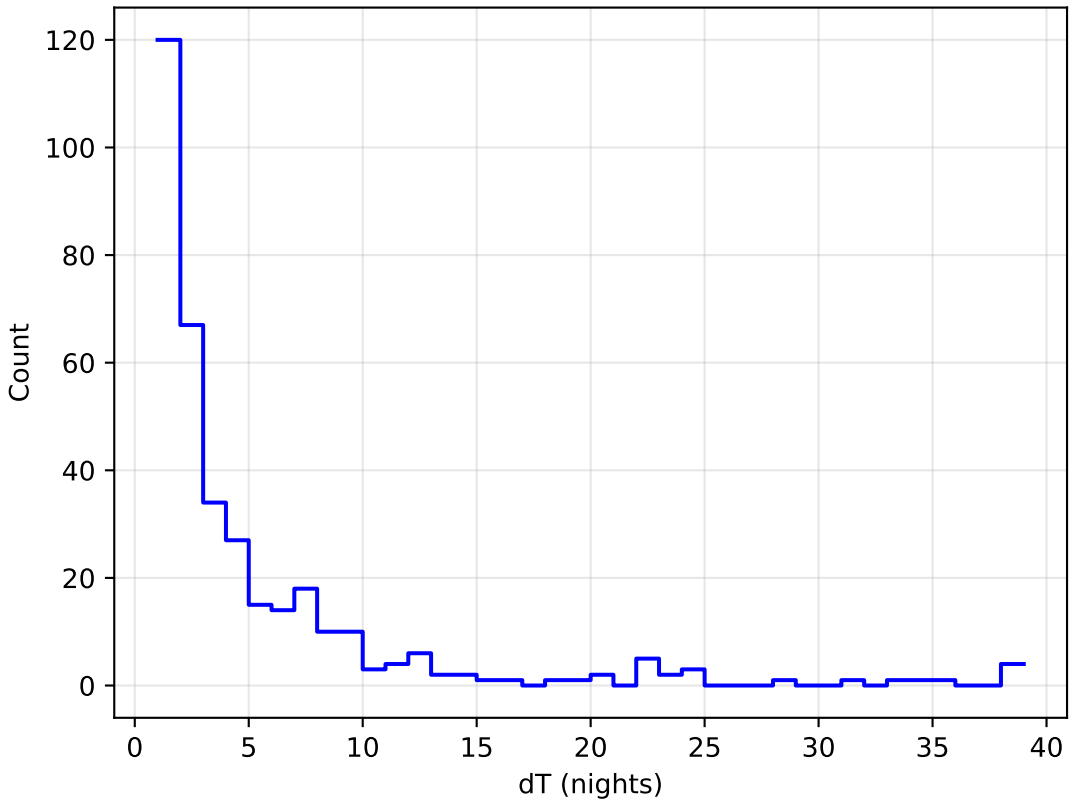
roman_v3.3_10yrs all bands: DD:WFD Delta Nights Histogram
