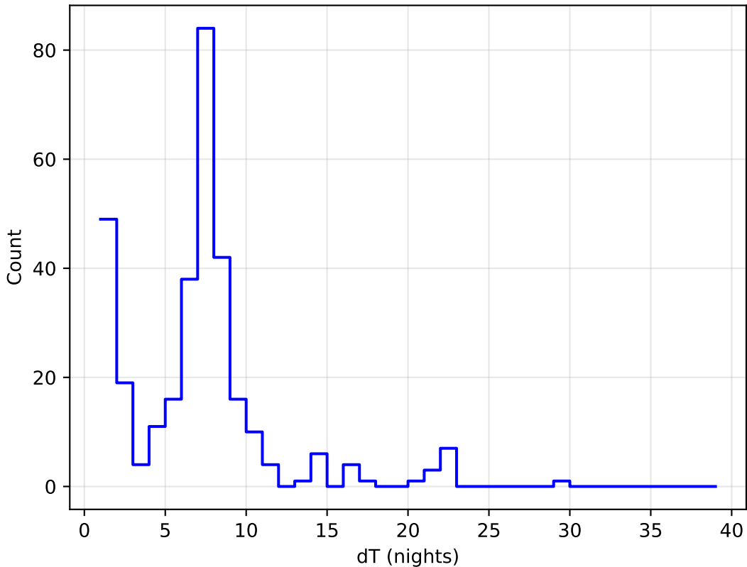
roman_v3.3_10yrs all bands: DD:EDFS Delta Nights Histogram
