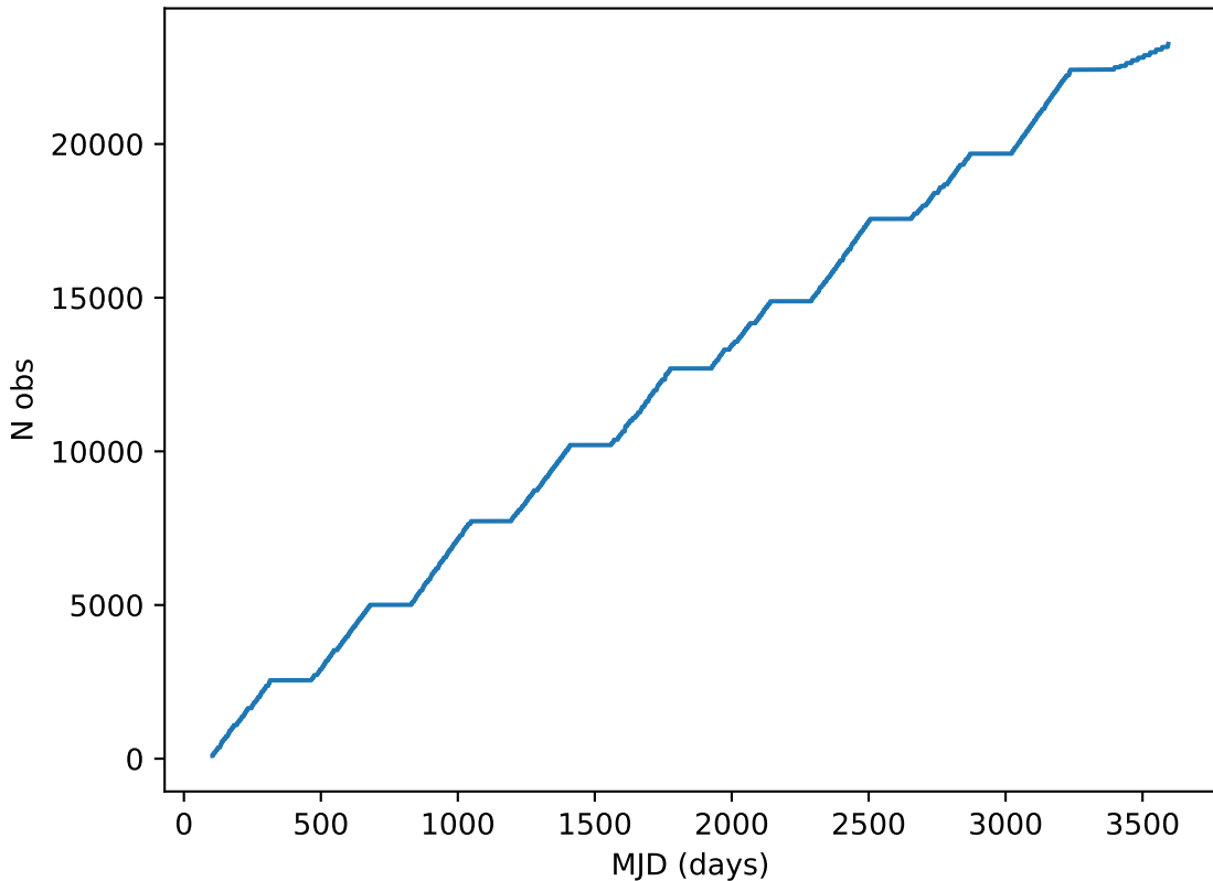
roman_v3.3_10yrs all bands: DD:EDFS Cumulative NVisits
