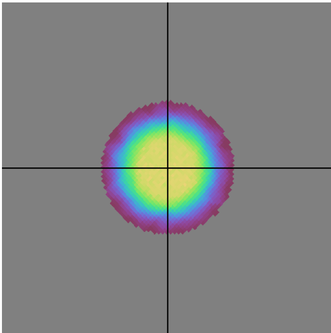
roman_v3.3_10yrs all bands: DD:ECDFS NVisits
