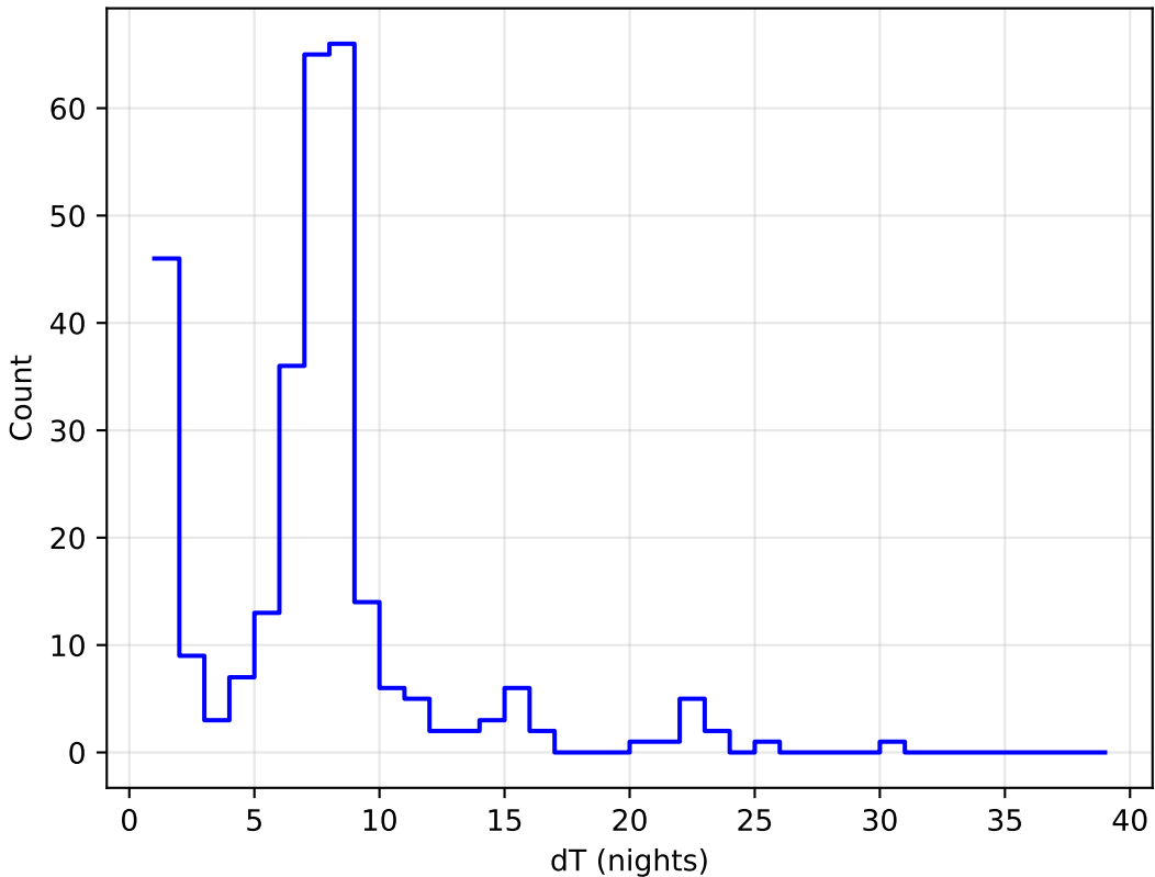
roman_v3.3_10yrs all bands: DD:ECDFS Delta Nights Histogram
