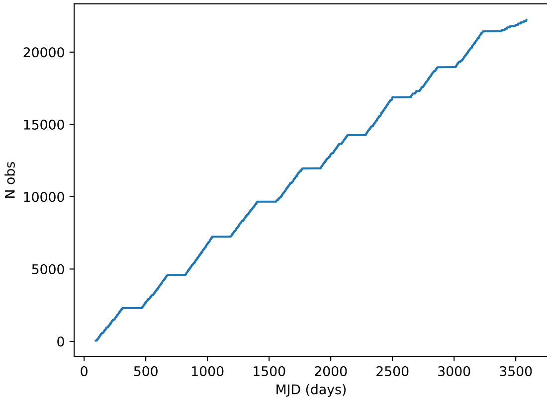
roman_v3.3_10yrs all bands: DD:ECDFS Cumulative NVisits
