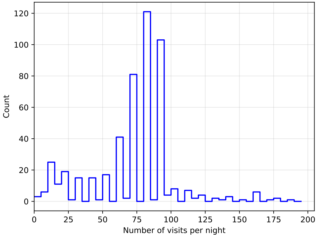
roman_v3.3_10yrs all bands: DD:COSMOS NVisitsPerNight
