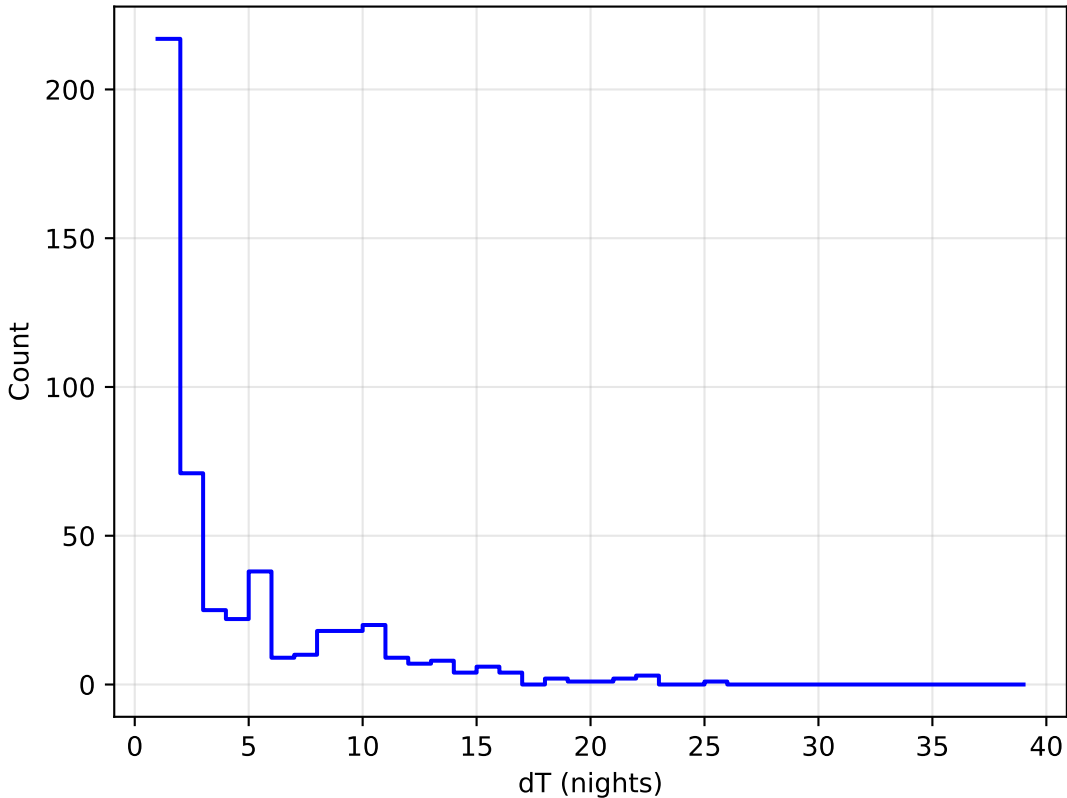
roman_v3.3_10yrs all bands: DD: COSMOS Delta Nights Histogram
