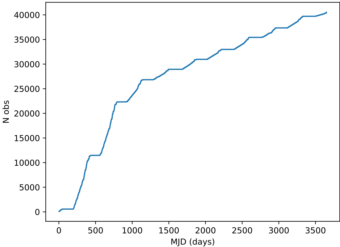
roman_v3.3_10yrs all bands: DD:COSMOS Cumulative NVisits
