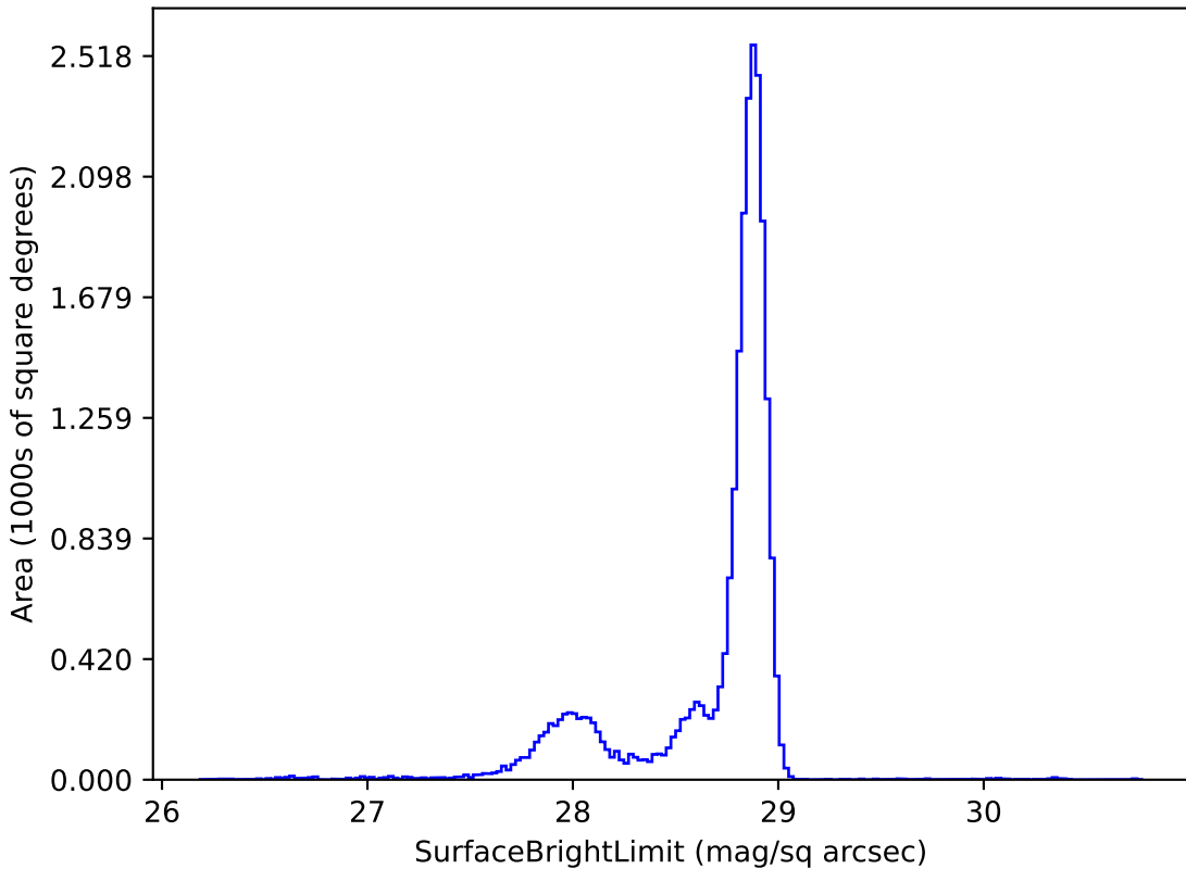
rolling_phased_ps_182_psf_91_v3.3_10yrs u: SurfaceBrightLimit
