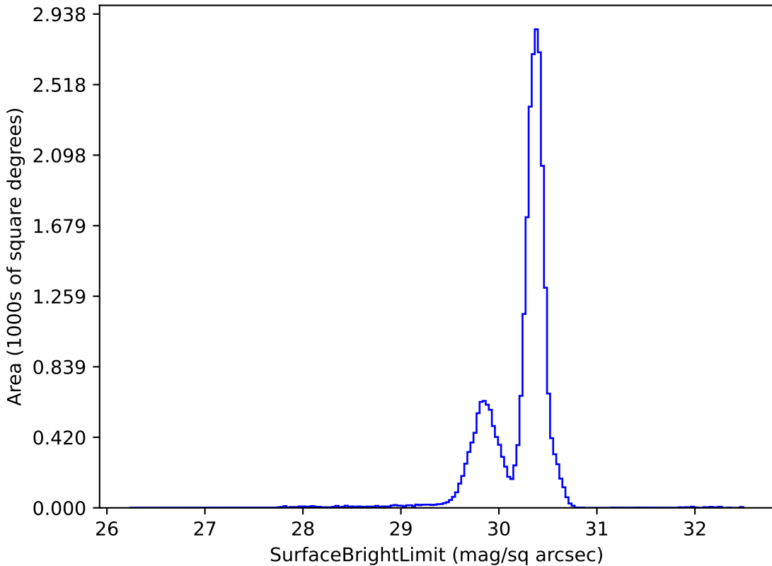
rolling_phased_ps_182_psf_91_v3.3_10yrs g: SurfaceBrightLimit
