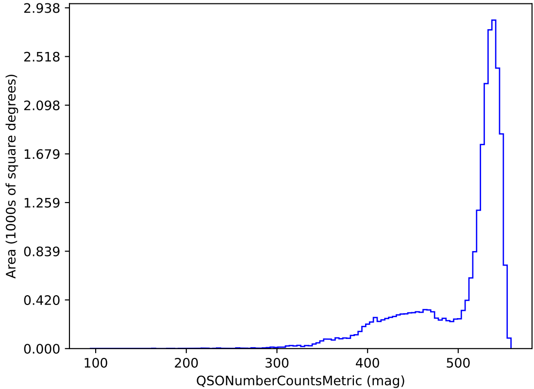
rolling_phased_ps_182_psf_91_v3.3_10yrs i band and non-DD: QSONumberCountsMetric
