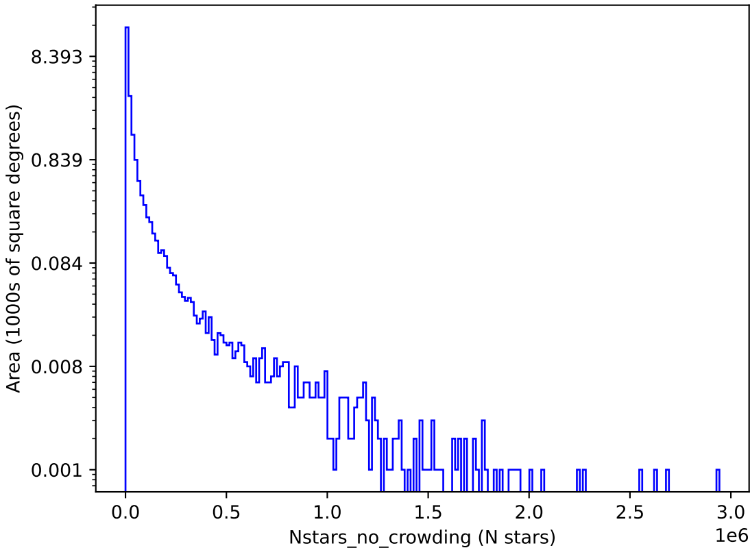
rolling_phased_ps_182_psf_91_v3.3_10yrs u: Nstars_no_crowding
